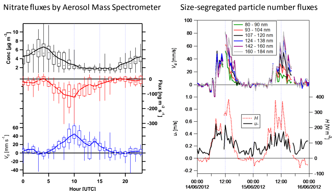
Figure 1.5: (a) Preliminary time-series of the concentrations, flux and deposition velocity of aerosol nitrate as measured by the Aerosol Mass Spectrometer flux system operated by NERC. (b) Preliminary time-series of the size segregated deposition velocity derived from particle number fluxes with an optical particle spectrometer (NERC, UGOT), in relation to heat flux ( H ) and friction velocity ( u^* ).
