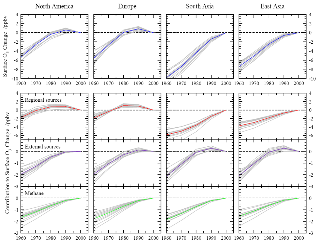
Figure 2.3: The HTAP model attribution of O 3 changes to Europe, North America, South Asia, and East Asia, to regional (domestic) sources; Rest-of-the-World and methane changes in emissions (Wild et al. 2010). This parameterisation was further developed to estimate future changes in ozone boundary conditions.
